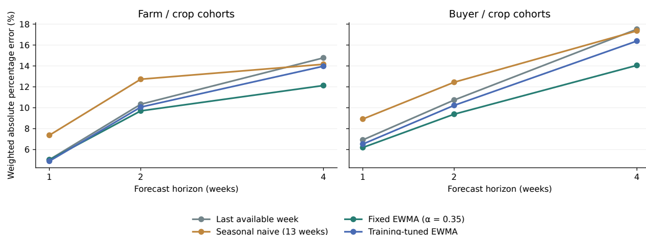
Figure 2. Current V4 rolling-origin synthetic demand results. The figure covers the two synthetic cohort levels and declared horizons; it contains no observed customer or farm demand.
