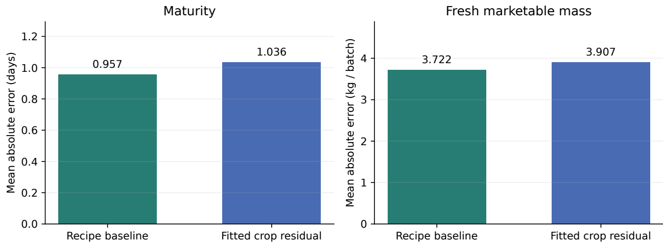
Figure 3. Independent synthetic crop-cycle evaluation. The fitted residual candidate fails to improve the primary MAE results and is not promoted.
