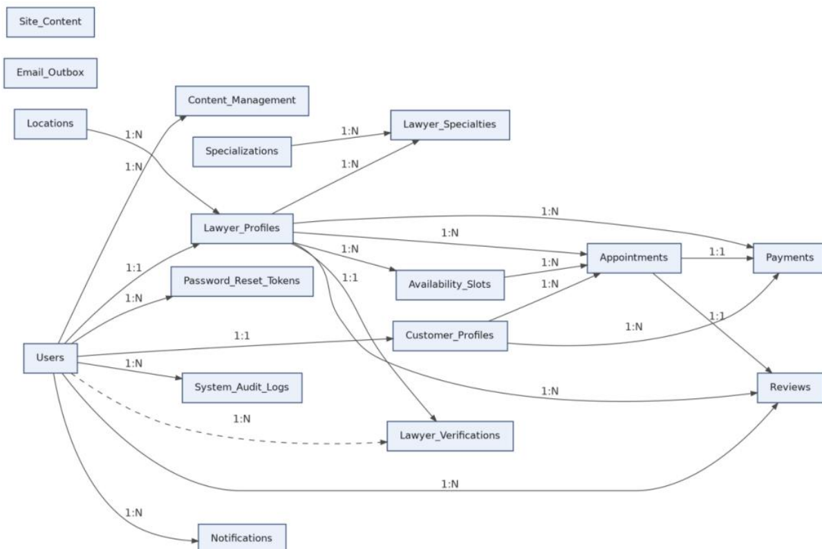
Figure 6. Entity–Relationship Diagram – LegalEase Database
