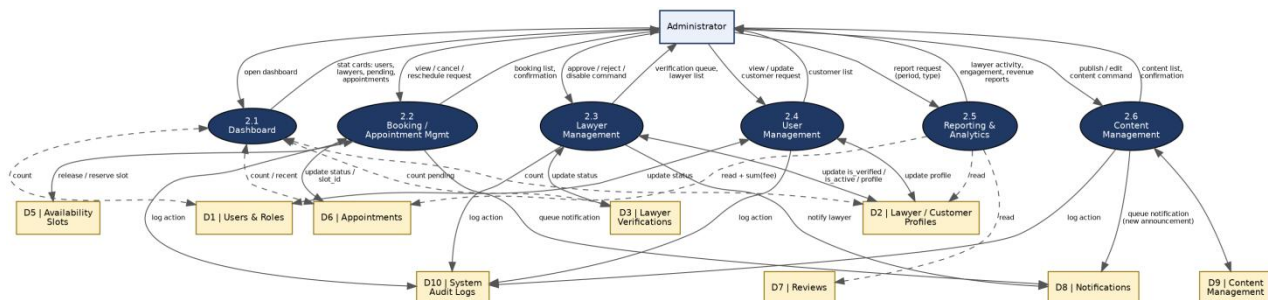
Figure 3. DFD Level 2 – Decomposition of Process 2.0 (Admin Features)
