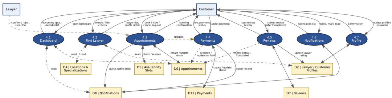
Figure 5. DFD Level 2 – Decomposition of Process 4.0 (Customer Features)
