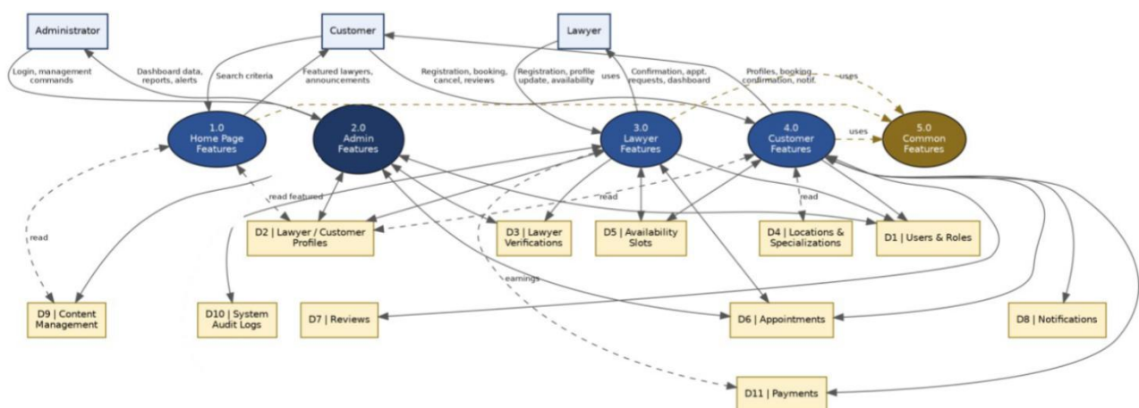
Figure 2. DFD Level 1 – Functional Overview of the LegalEase System
