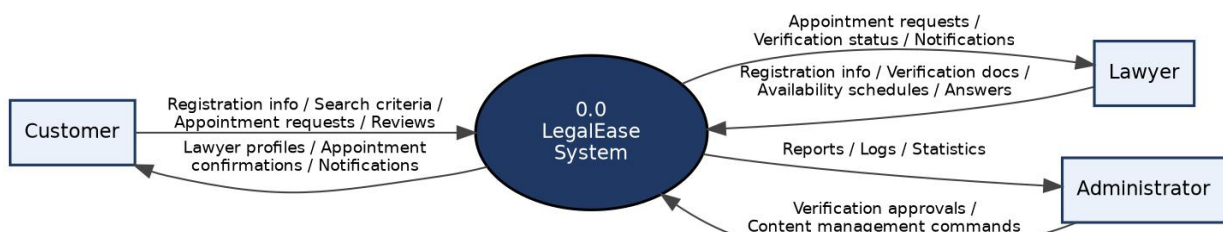
Figure 1. DFD Level 0 – Context Diagram of the LegalEase System
