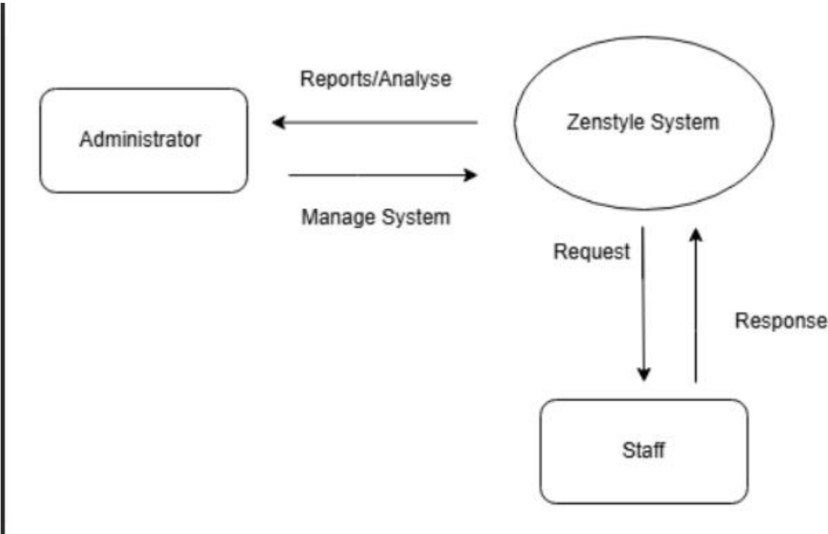
Figure 1: DFD level 0
