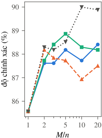
Ionosphere
