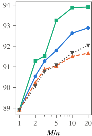
Spambase
