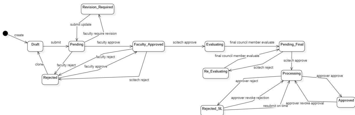
Picture Error: Reference source not found-18 Initiative statechart diagram
