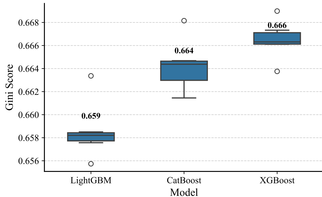
Gini Distribution Across Folds
