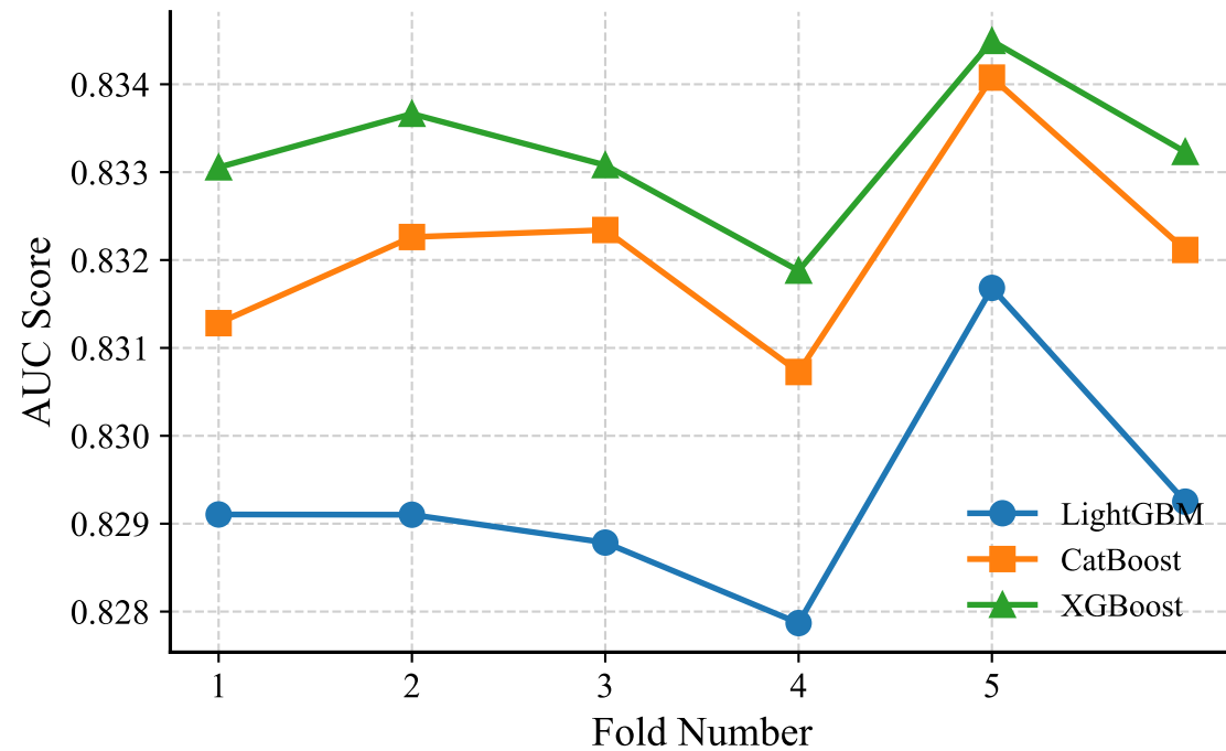
AUC Across Folds
