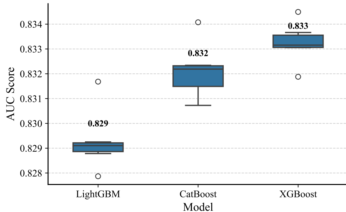
AUC Distribution Across Folds
