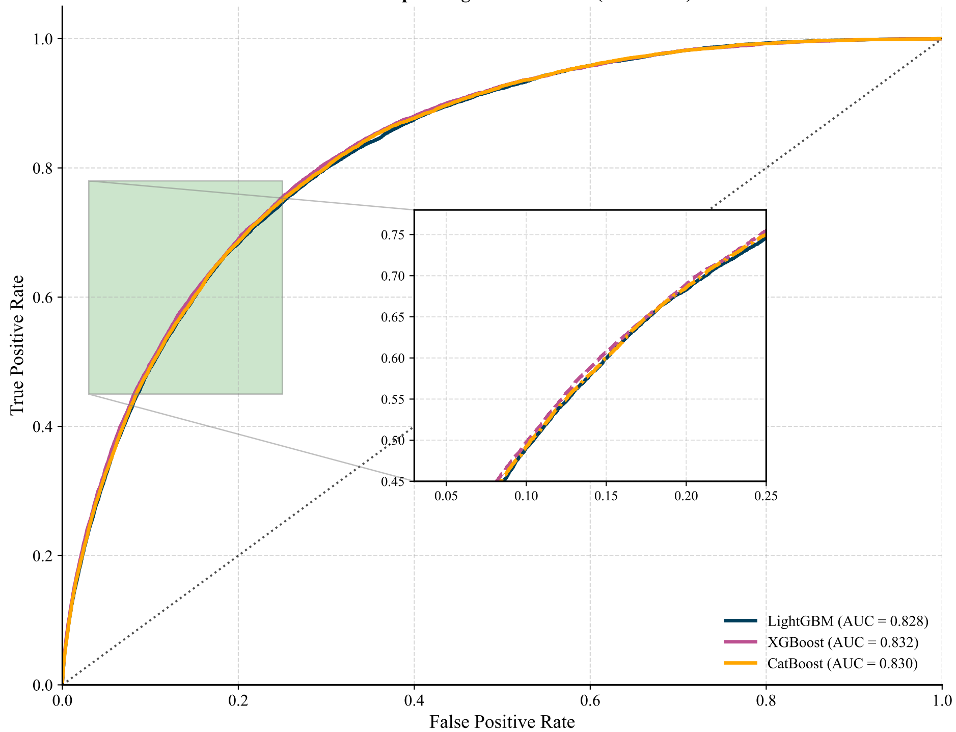
Receiver Operating Characteristic (Validation)
