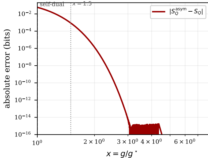
(b) Entropy asymptotic
