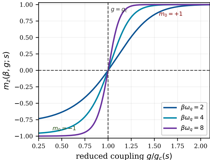
(b) Universal finite- \beta sharpening
