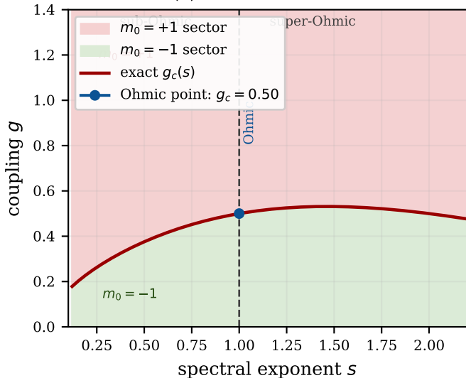
(a) Exact critical line
