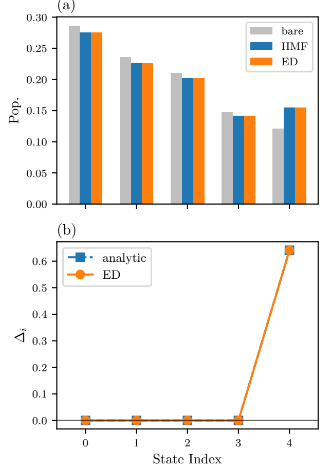
FIG. 4. Microscopic validation. (a) Detailed population snapshot at fixed \beta, g : Analytic HMF (blue) corrects the bare Gibbs (grey) to match ED (orange). (b) Effective energy shifts \Delta_i for each level; only the coupled level ( |4\rangle ) shifts, by exactly -\lambda . Non-coupled levels remain unperturbed.
