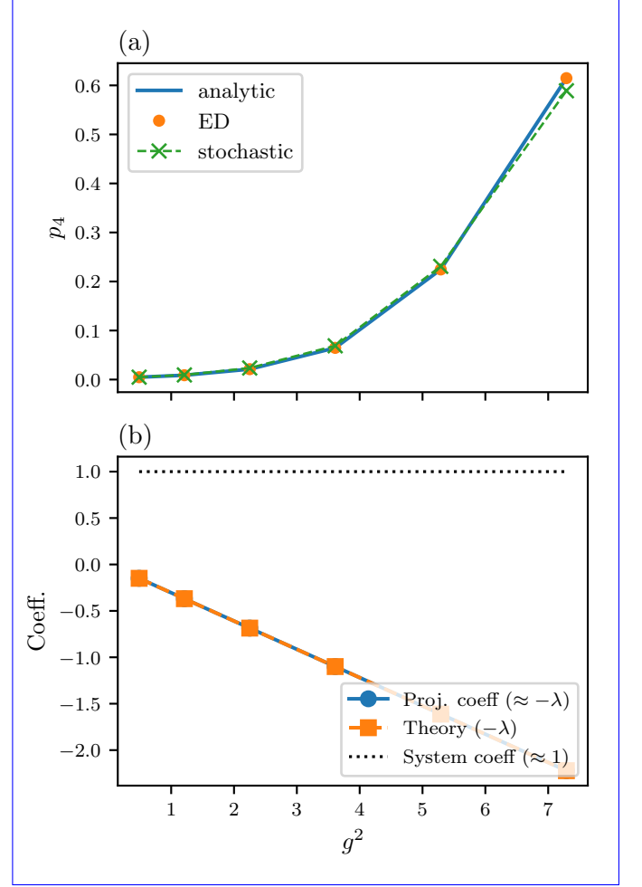
FIG. 3. Strong-coupling benchmark. (a) Population p_4 vs g^2 at fixed \beta , showing excellent agreement over the full range. (b) Coefficients in the system basis vs g^2 . The projector component P_4 = |4\rangle\langle 4| scales as -\lambda , while off-diagonal coherences are exponentially suppressed. This strong-coupling projector dominance is consistent with ultrastrong-coupling analyses of the mean-force Gibbs state [18]. The bare system Hamiltonian H_S remains unrenormalised (dotted), confirming H_{\text{MF}} = H_S - \lambda f^2 .
