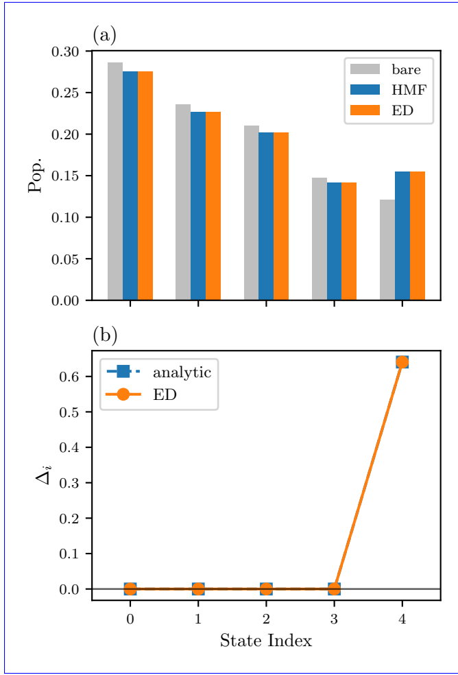
FIG. 4. Microscopic validation. (a) Detailed population snapshot at fixed \beta, g : “Analytic HMF” (blue) corrects the “Bare-bare” Gibbs (grey) to match ED (orange). (b) Effective energy shifts \Delta_i for each level; only the coupled level (|4>) shifts, by exactly -\lambda . Non-coupled levels remain unperturbed.
