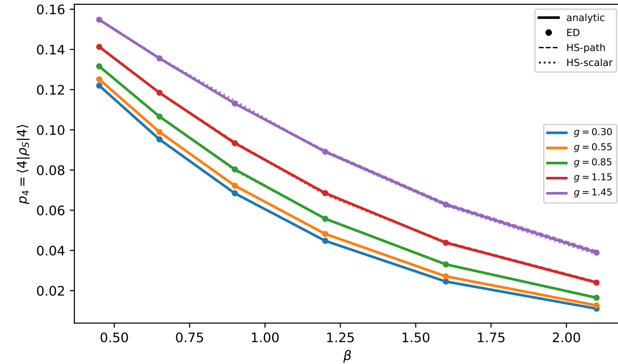
(A) Coupled-level population (cutoff=8)
