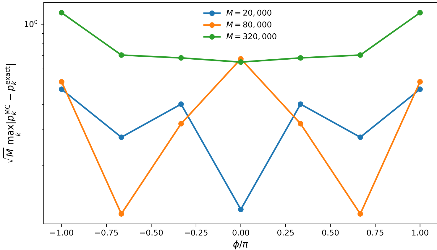
\sqrt{M} scaling collapse ( \tau_c = 0.12 , N = 18 )
