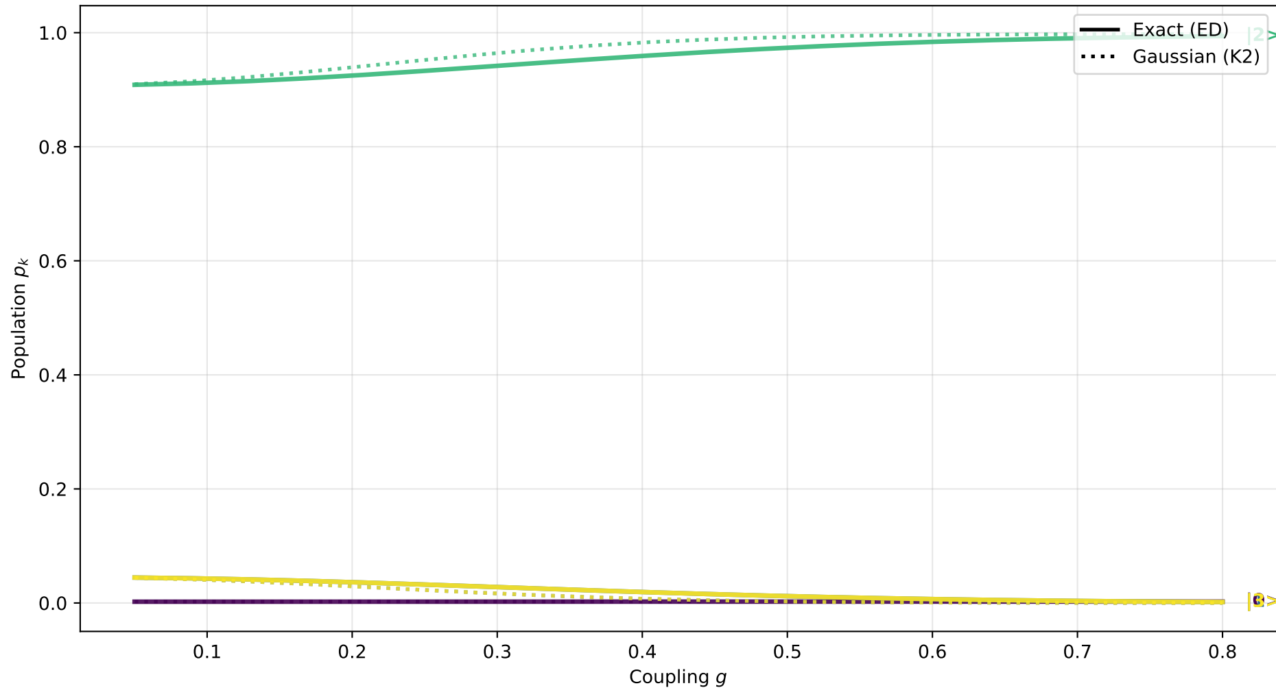
N=4 Clock Model, \beta = 2.5 (Low T) Freezing bath causes Gaussian failure
