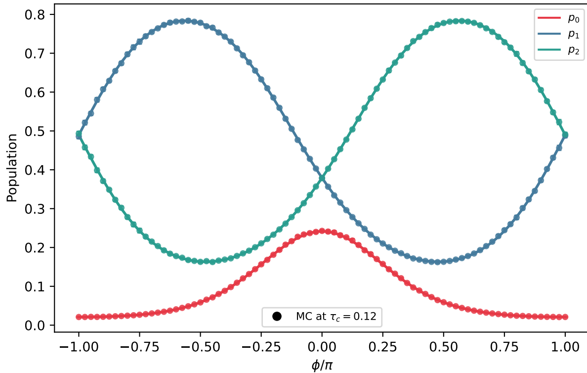
(A) Smooth analytic curves + MC overlays
