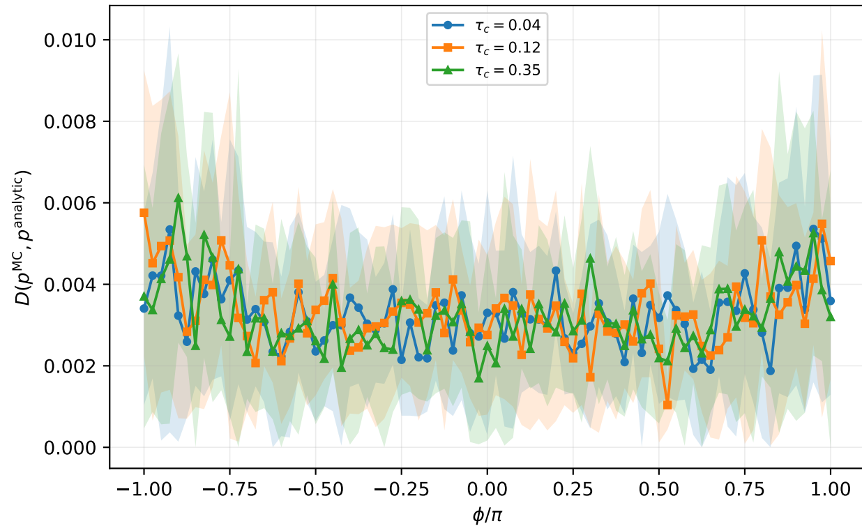
(B) Trace-distance error across phase
