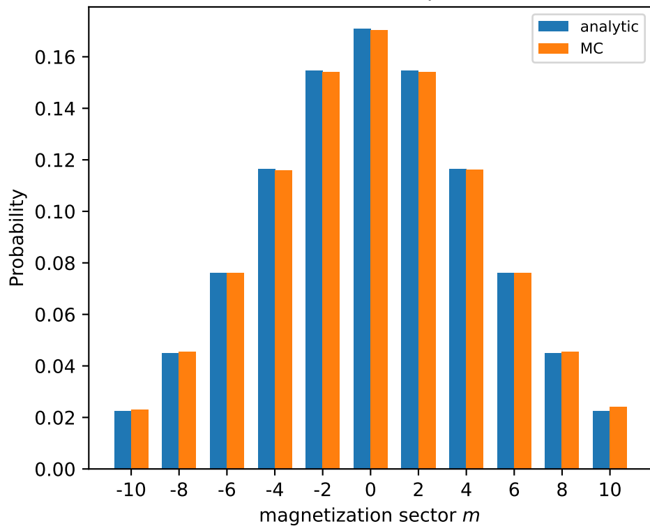
(A) PSD branch (multi-qubit sectors)
