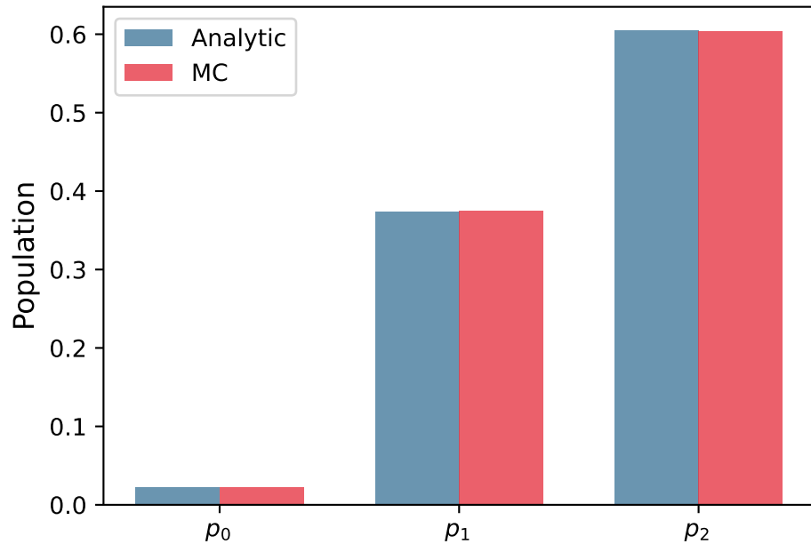
Non-PSD stress test ( \phi = 0.9\pi )
