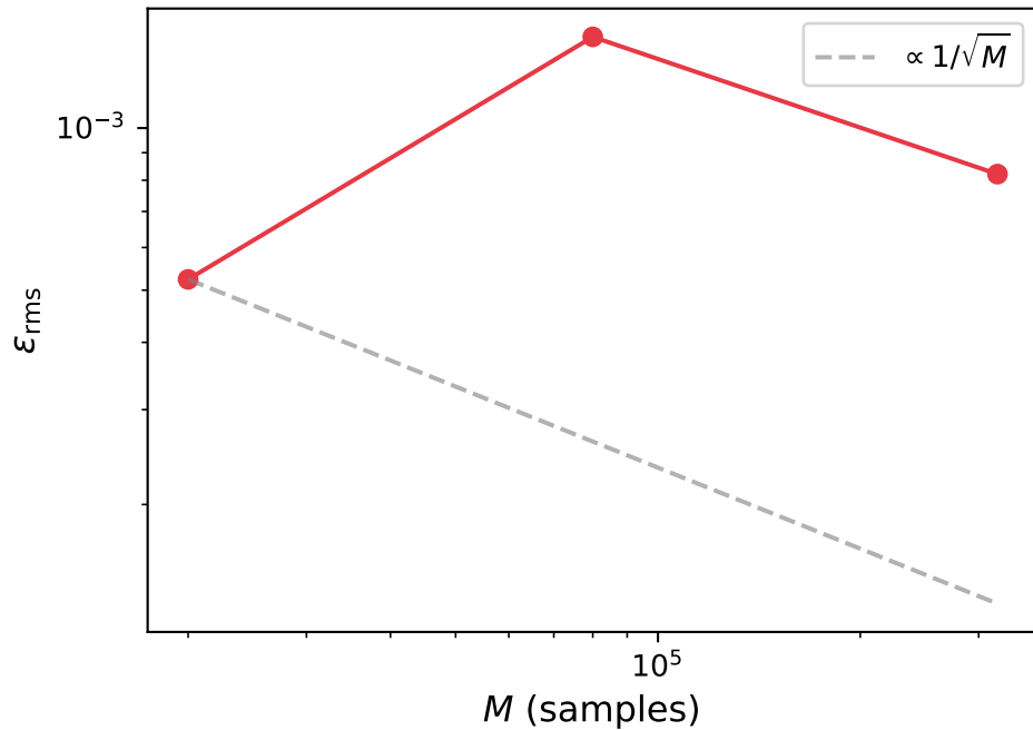
Error scaling at \phi = 0.9\pi
