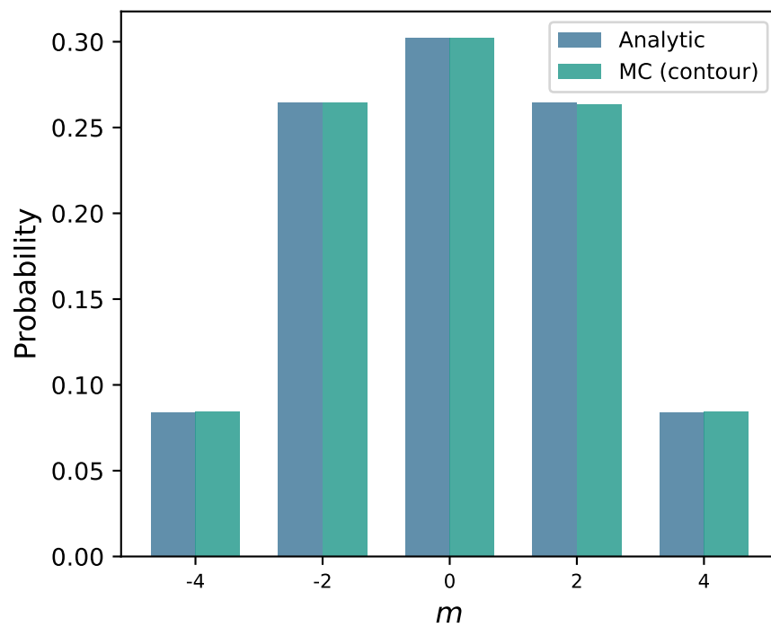
Non-PSD: k_2 = 0.08 , k_4 = -0.003
