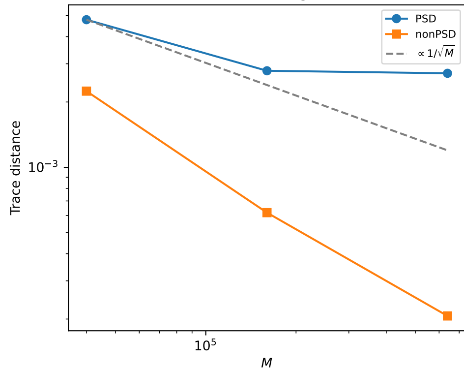
(C) MC convergence
