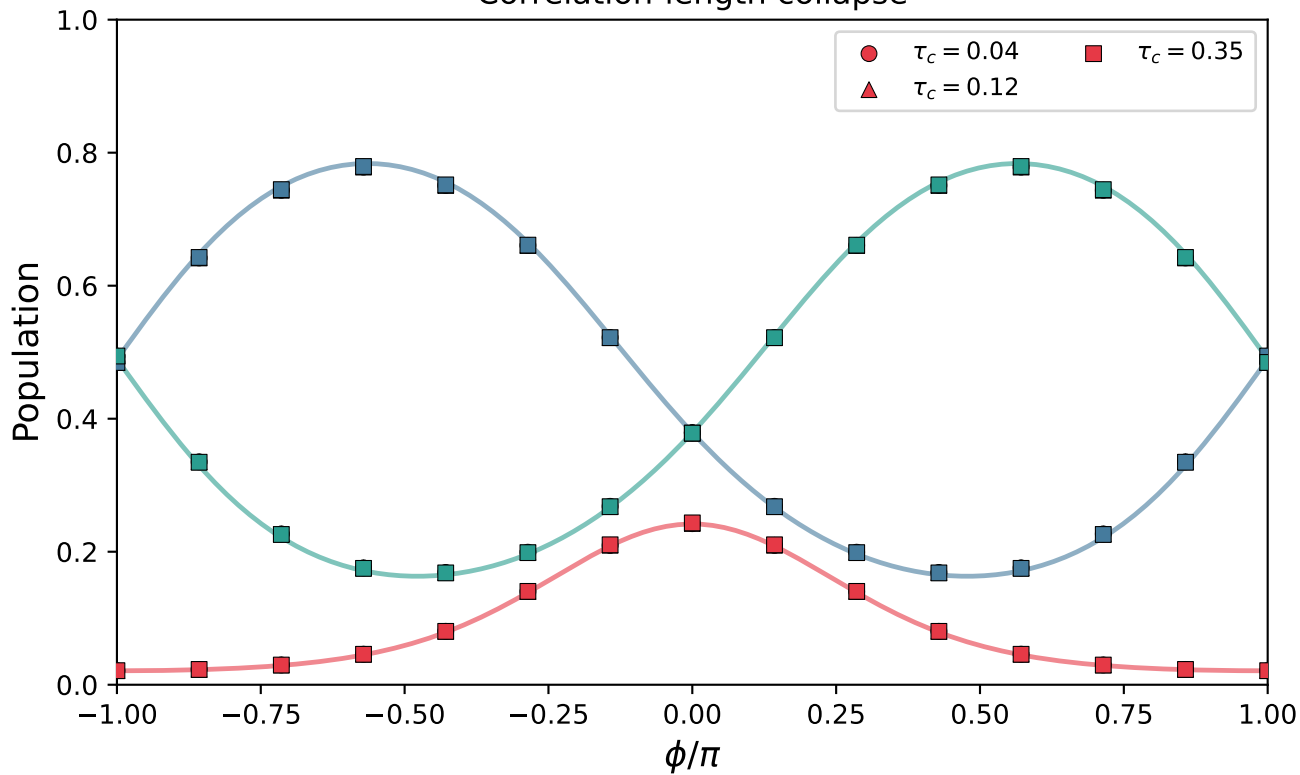
Correlation-length collapse
