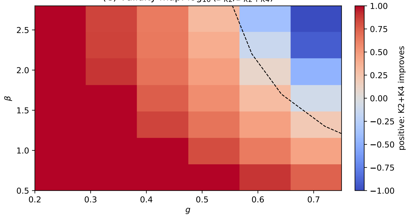
(C) Validity map: \log_{10}(D_{K2}/D_{K2+K4})
