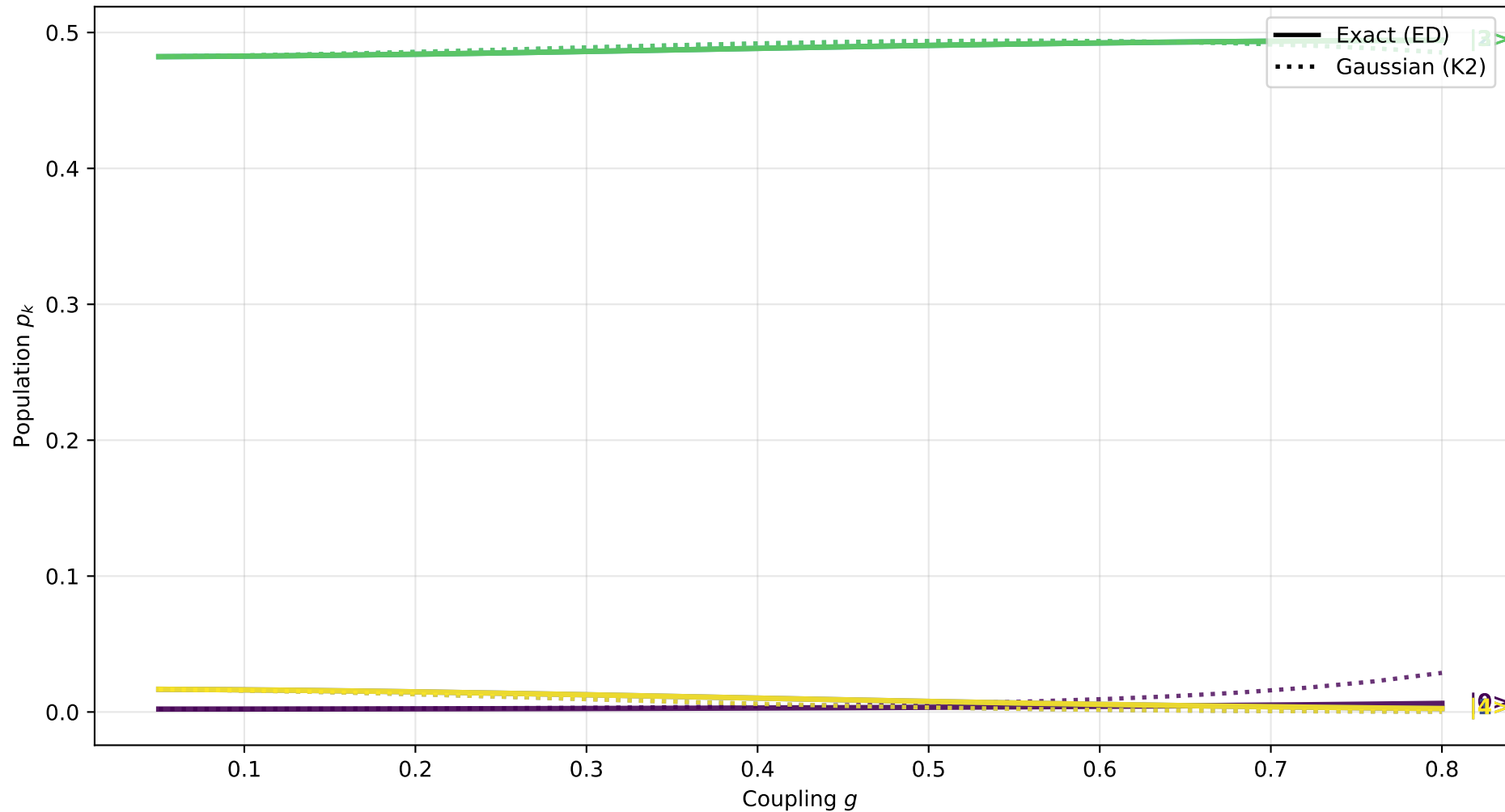
N=5 Clock Model, \beta = 2.5 (Low T) Freezing bath causes Gaussian failure
