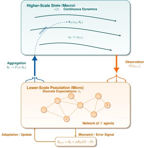
FIG. 2. The Multiscale Adaptive Loop. The canonical structural cycle driving upper-lower multiscale systems. A vast population of lower-scale agents forms local expectations \theta_k regarding a macroscopic state variable x(t) . These individual actions aggregate into a collective signal that periodically reparametrises the constraints governing the higher-scale continuous dynamics. The accumulated state O(x_{k+1}) is subsequently broadcast downward to drive the next expectation update. Crucially, this direct feedback loop lacks hierarchical filtering, rendering the macroscopic state vulnerable to systemic instabilities.
