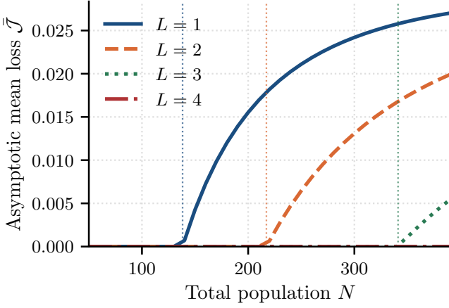
FIG. 6. Hierarchical Attenuation of the Thermodynamic Divergence. As the total population N scales, unmediated flat systems ( L = 1 ) rapidly cross the stability boundary and diverge into catastrophic loss. The insertion of successive hierarchical layers exponentially attenuates the macroscopic gain, thereby preserving the stable modular phase for exponentially larger critical population sizes.
