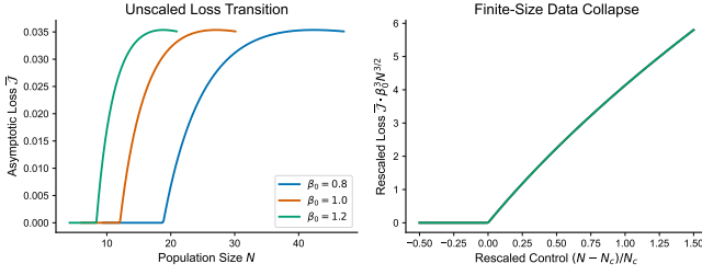
FIG. 3. Finite-Size Data Collapse. The asymptotic loss \bar{\mathcal{J}} emerges continuously above the critical population size N_c (left). When appropriately rescaled, the disparate loss curves collapse onto a single universal form defined by the mean-field exponent \beta = 1/2 (right), confirming the transition as a macroscopic phase boundary.
