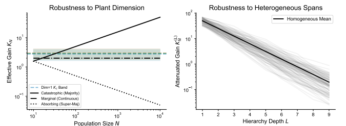
FIG. 11. Robustness of the Universality Classes. (A) For higher-dimensional plants, the exact stability boundary shifts but remains bounded \mathcal{O}(1) . The \sqrt{N} divergence of the catastrophic class inevitably crosses it, while marginal and absorbing rules do not. (B) Heterogeneous layer spans introduce variance but preserve the exponential attenuation required to stabilise the macroscopic gain.
