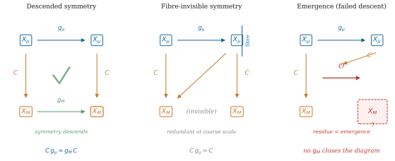
FIG. 9. Transported symmetry, fibre-invisible symmetry, and failed closure (appendix figure). Left: Fine symmetry satisfying Cg_\mu = g_M C ; transported symmetry. Centre: Fine transformation satisfying Cg_\mu = C ; fibre-invisible, becomes gauge redundancy. Right: No g_M closes the diagram; failed closure—residue is emergence.
