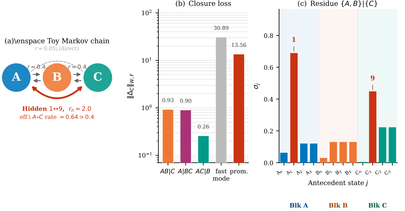
FIG. 8. Constructive coarse-graining demonstration. (a) Schematic of the 12-state CTMC. Blocks A, B, C each have fast internal equilibration ( r = 30 hub \rightarrow spoke, r = 12 inward). Slow inter-block hub-to-hub connections ( r = 0.4 , grey) suggest a chain topology. A hidden shortcut between spoke states 1 \in A and 9 \in C (red, r = 2.0 ) raises the effective A - C coupling to \approx 0.64 , exceeding the inter-block rate and making A and C dynamically closer than either is to B . (b) Closure loss \|\Delta_C\|_{W,F} for candidate coarse-grainings (log scale). \{A, C\} \mid \{B\} (teal) achieves the minimum loss 0.26; topology-guided partitions score 0.93 and 0.90; fast-mode compression scores 30.9. (c) Weighted column profile \sigma_j for the wrong partition \{A, B\} \mid \{C\} . States 1 and 9 (red bars) spike by a factor of \sim 6 above all other contributors, identifying the hidden-shortcut endpoints without prior knowledge of the shortcut.
