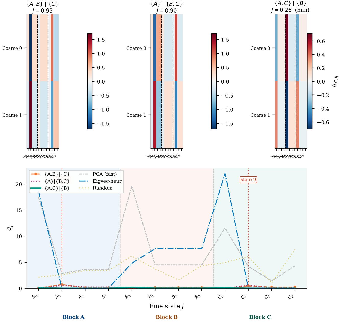
FIG. 13. Closure residue anatomy for candidate bases. Top row: Heatmaps of \Delta_C = CG_\mu - G_M^*C for the three binary block partitions. The two topology-guided partitions carry large, spatially coherent residue; \{A, C\} | \{B\} carries small, diffuse residue (closure losses 0.26 vs. 0.93 and 0.90). Bottom panel: Weighted column profile \sigma_j for all three 2-state partitions. For \{A, B\} | \{C\} , states 1 and 9 stand out by a factor of \sim 6 above the next contributor: these are the hidden-shortcut endpoints, identified by residue anatomy without prior knowledge of the shortcut. For \{A, C\} | \{B\} , the profile is uniformly small and structureless, indicating an adequate representation.
