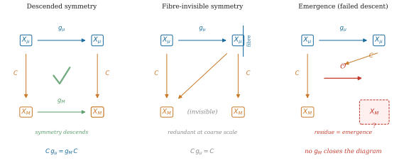
FIG. 10. Transported symmetry, fibre-invisible symmetry, and failed closure (appendix figure). Left: Fine symmetry satisfying Cg_\mu = g_M C ; transported symmetry. Centre: Fine transformation satisfying Cg_\mu = C ; fibre-invisible, becomes gauge redundancy. Right: No g_M closes the diagram; failed closure—residue is emergence.
