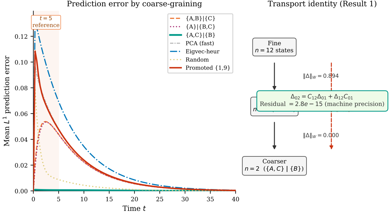
FIG. 14. Prediction accuracy and the transport identity. Left: Mean L^1 prediction error \mathbb{E}_\rho[\|Ce^{tG_\mu}\rho - e^{tG_M^*}C\rho\|_1] versus time for all candidate coarse-grainings (averaged over 50 random initial distributions \rho ). \{A, C\} | \{B\} (teal, solid) outperforms all 2-state alternatives by 65–80 \times at t = 5 and improves further at t = 20 . The fast-mode heuristic (light grey) and slow-mode heuristic (blue, dot-dash) perform no better than the wrong topological partitions, confirming that spectral contamination defeats both heuristics while J(C) is unaffected. Right: The three-scale transport identity \Delta_{C02} = C_{12}\Delta_{C01} + \Delta_{C12}C_{01} (Result 3) verified numerically for the tower 12 \rightarrow 3 \rightarrow 2 ; residual 2.83 \times 10^{-15} at machine precision.
