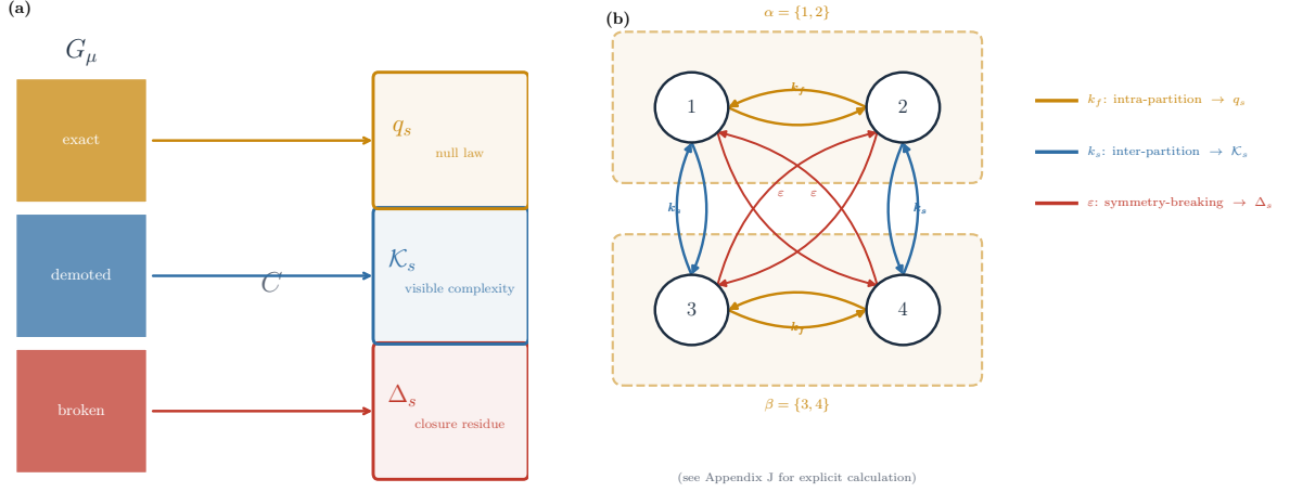
FIG. 3. Coarse-graining sorts the symmetry content of a generator. (a) The fine generator G_\mu contains three classes of structure, distinguished by how the coarse-graining C acts on them. Exact symmetries are absorbed into the null law q_s (amber); demoted symmetries become visible constraints entering \mathcal{K}_s (blue); broken structure has no coarse image and contributes to the closure residue \Delta_s (red). (b) A four-state Markov chain with coarse partition \alpha = \{1, 2\} , \beta = \{3, 4\} instantiates all three fates explicitly. Intra-partition transitions at rate k_f (amber) equilibrate instantly inside each partition and are absorbed into the null law q_s . Inter-partition transitions at rate k_s (blue) project cleanly through C and enter \mathcal{K}_s as explicit constraints. Diagonal transitions at rate \varepsilon (red) break the partition symmetry and cannot be expressed in any coarse functional, contributing to \Delta_s . Full derivation in Appendix J.
