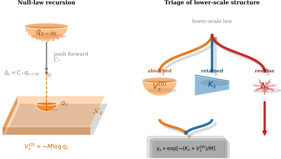
FIG. 6. Null law recursion and residue triage. Left: The finer null law q_{s-ds} is pushed forward through C to give \hat{q}_s = C_* q_{s-ds} , then projected onto the admissible class \mathcal{N}_s to give q_s (amber, Eq. 4). The inherited null potential V_s^{(0)} = -M \log q_s (amber) is the lower-scale law structure absorbed into the current-scale background. The visible deformation K_s (blue) is resolved structure remaining after absorption; their sum K_s + V_s^{(0)} is the total effective generator. Right: The triage of lower-scale law (Eq. 11). Every part of the lower-scale law is either absorbed (amber), retained (blue), or left as closure residue (red). Recursive null-law derivation in Appendix B.
