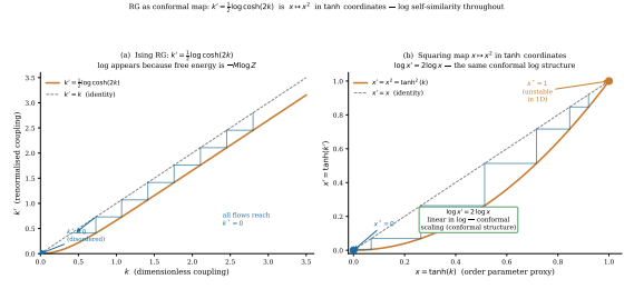
FIG. 12. Ising RG as conformal map (appendix figure). Left: Cobweb diagram for the 1D Ising recursion k' = \frac{1}{2} \log \cosh(2k) . Right: In \tanh coordinates the recursion is the squaring map x \mapsto x^2 , which is linear in log-coordinates. The logarithm appears because it is the generator flow inside the invariant free-energy form.
