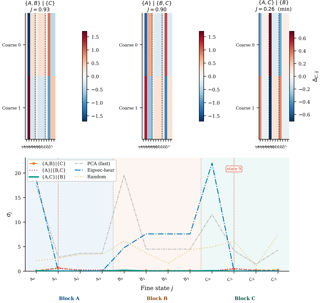
FIG. 10. Closure residue anatomy for candidate bases. Top row: Heatmaps of \Delta_C = CG_\mu - G_M^*C for the three binary block partitions. The two topology-guided partitions carry large, spatially coherent residue; \{A, C\} | \{B\} carries small, diffuse residue (closure losses 0.26 vs. 0.93 and 0.90). Bottom panel: Weighted column profile \sigma_j (Eq. 19) for all three 2-state partitions. For \{A, B\} | \{C\} , states 1 and 9 stand out by a factor of \sim 6 above the next contributor: these are the hidden-shortcut endpoints, identified by residue anatomy without prior knowledge of the shortcut. For \{A, C\} | \{B\} , the profile is uniformly small and structureless, indicating an adequate representation.
