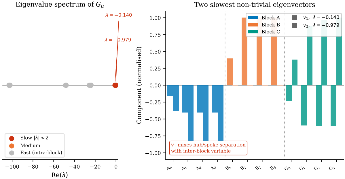
FIG. 9. Eigenvalue spectrum and slow eigenvectors of G_\mu . Left : The 12 eigenvalues on the real line. Two slow modes ( \lambda \approx -0.14 and \lambda \approx -0.98 , red) are separated by a spectral gap from the fast intra-block modes (grey). Right : Components of the two slowest eigenvectors over all 12 states, coloured by block membership. The slowest mode ( \lambda \approx -0.14 ) is contaminated by the within-block hub/spoke asymmetry induced by the hidden shortcut; it separates spoke states from hub states across all three blocks, not block A \cup C from block B . A threshold-based heuristic using this eigenvector therefore fails to recover \{A, C\} \mid \{B\} , while the direct criterion J(C) is unaffected.
