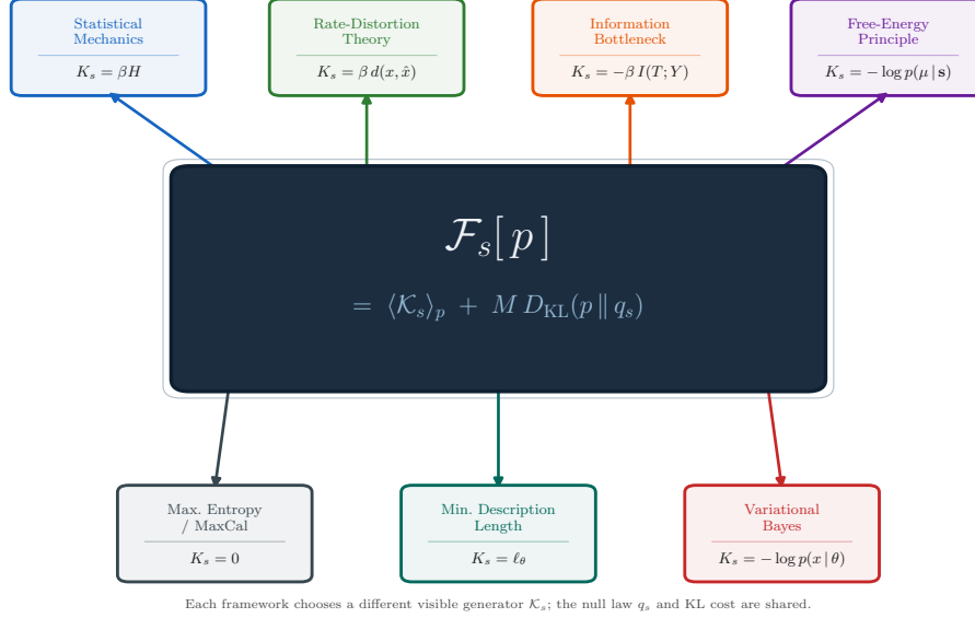
FIG. 5. The forced law-form unifies seven variational frameworks. The free-energy functional \mathcal{F}_s[p] = \langle K_s \rangle_p + MD_{\text{KL}}(p||q_s) (centre) is shared by all seven frameworks. Each spoke chooses a different visible generator K_s ; the null law q_s and the KL cost are common to all. Thermodynamics takes K_s = \beta H ; rate-distortion theory [3] takes distortion; the information bottleneck [5] takes relevance gap; the free-energy principle [19] takes prediction error on a Markov blanket; Rissanen’s MDL [6] takes code length; variational Bayes takes negative log-likelihood; MaxEnt [1] takes no visible constraint ( K_s = 0 ) and returns directly to the null law. The correspondences are not analogies but identifications within a single forced structure. Every framework in the figure is the case where order independence holds: partition and accounting commute, and the KL form is uniquely forced.
