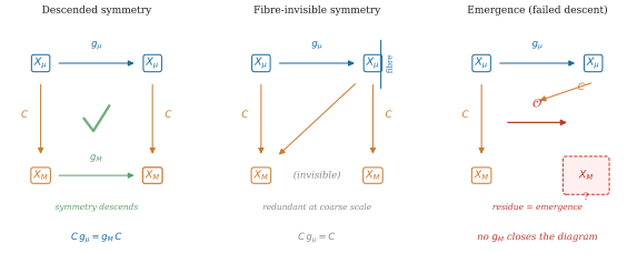
FIG. 13. Transported symmetry, fibre-invisible symmetry, and failed closure (appendix figure). Left: Fine symmetry satisfying Cg_\mu = g_M C ; transported symmetry. Centre: Fine transformation satisfying Cg_\mu = C ; fibre-invisible, becomes gauge redundancy. Right: No g_M closes the diagram; failed closure—residue is emergence.
