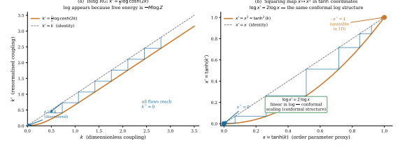
FIG. 12. Ising RG as conformal map (appendix figure). Left: Cobweb diagram for the 1D Ising recursion k' = \frac{1}{2} \log \cosh(2k) . Right: In \tanh coordinates the recursion is the squaring map x \mapsto x^2 , which is linear in log-coordinates. The logarithm appears because it is the generator flow inside the invariant free-energy form.
