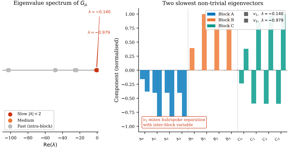
FIG. 9. Eigenvalue spectrum and slow eigenvectors of G_\mu . Left: The 12 eigenvalues on the real line. Two slow modes ( \lambda \approx -0.14 and \lambda \approx -0.98 , red) are separated by a spectral gap from the fast intra-block modes (grey). Right: Components of the two slowest eigenvectors over all 12 states, coloured by block membership. The slowest mode ( \lambda \approx -0.14 ) is contaminated by the within-block hub/spoke asymmetry induced by the hidden shortcut; it separates spoke states from hub states across all three blocks, not block A \cup C from block B . A threshold-based heuristic using this eigenvector therefore fails to recover \{A, C\} \mid \{B\} , while the direct criterion J(C) is unaffected.
