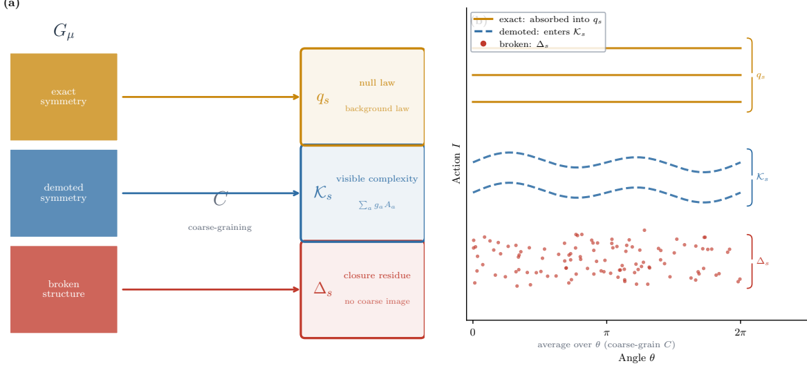
FIG. 3. Coarse-graining sorts the symmetry content of a generator. (a) The fine generator G_\mu contains three classes of structure, distinguished by how the coarse-graining C acts on them. Exact symmetries are absorbed into the null law q_s (amber); demoted symmetries become visible constraints entering \mathcal{K}_s (blue); broken structure has no coarse image and contributes to the closure residue \Delta_s (red). (b) In action-angle coordinates (I, \theta) , the three classes correspond to orbits at different action values. Coarse-graining averages over \theta ; orbits at high action (exact conserved quantities, amber) survive as null-law structure; orbits at intermediate action (demoted, blue) enter \mathcal{K}_s as explicit constraints; orbits at low action (broken, red) have no stable coarse image and contribute to the residue.
