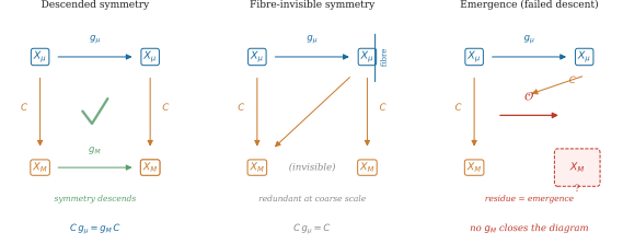
FIG. 9. Transported symmetry, fibre-invisible symmetry, and failed closure (appendix figure). Left: Fine symmetry satisfying Cg_\mu = g_M C ; transported symmetry. Centre: Fine transformation satisfying Cg_\mu = C ; fibre-invisible, becomes gauge redundancy. Right: No g_M closes the diagram; failed closure—residue is emergence.
