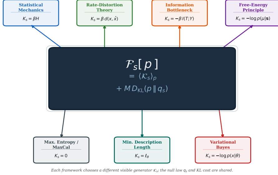
FIG. 5. The forced law-form unifies seven variational frameworks. The free-energy functional \mathcal{F}_s[p] = \langle K_s \rangle_p + MD_{\text{KL}}(p \parallel q_s) (centre) is shared by all seven frameworks. Each spoke chooses a different visible generator K_s ; the null law q_s and the KL cost are common to all. Thermodynamics takes K_s = \beta H ; rate-distortion theory [3] takes distortion; the information bottleneck [5] takes relevance gap; the free-energy principle [18] takes prediction error on a Markov blanket; Rissanen’s MDL [6] takes code length; variational Bayes takes negative log-likelihood; MaxEnt [1] takes no visible constraint ( K_s = 0 ) and returns directly to the null law. The correspondences are not analogies but identifications within a single forced structure.
