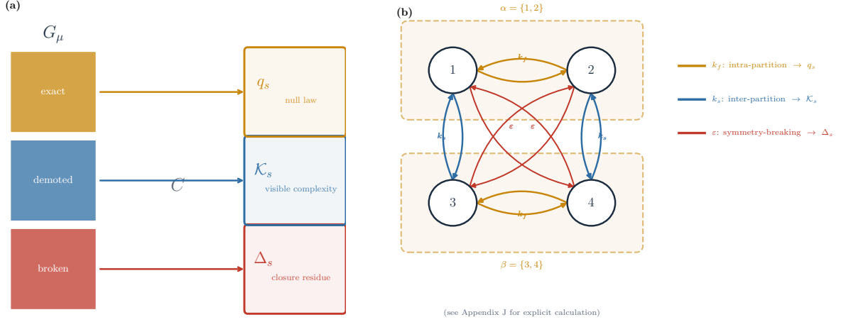
FIG. 3. Coarse-graining sorts the symmetry content of a generator. (a) The fine generator G_\mu contains three classes of structure, distinguished by how the coarse-graining \mathcal{C} acts on them. Exact symmetries are absorbed into the null law q_s (amber); demoted symmetries become visible constraints entering \mathcal{K}_s (blue); broken structure has no coarse image and contributes to the closure residue \Delta_s (red). (b) In action-angle coordinates (I, \theta) , the three classes correspond to orbits at different action values. Coarse-graining averages over \theta ; orbits at high action (exact conserved quantities, amber) survive as null-law structure; orbits at intermediate action (demoted, blue) enter \mathcal{K}_s as explicit constraints; orbits at low action (broken, red) have no stable coarse image and contribute to the residue.
