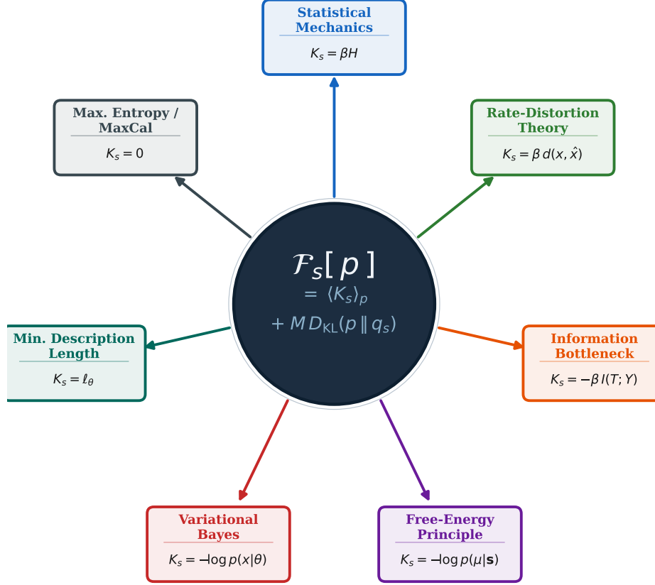
Each spoke assigns a different visible generator K_s ; the null law q_s and KL cost are shared.
