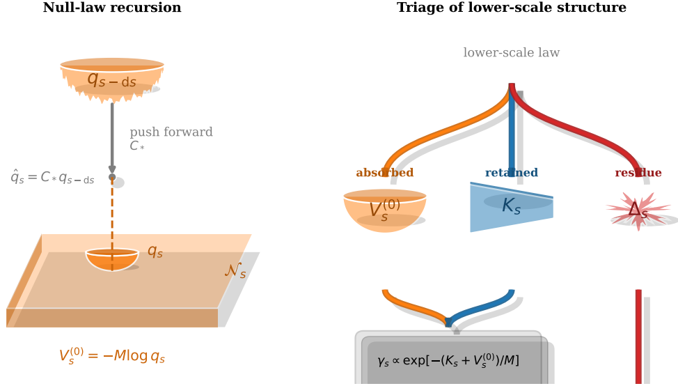
FIG. 5. Null law recursion and residue triage. Left: The finer null law q_{s-ds} is pushed forward through C to give \hat{q}_s = C_* q_{s-ds} , then projected onto the admissible class \mathcal{N}_s to give q_s (amber, Eq. 8). The inherited null potential V_s^{(0)} = -M \log q_s (amber) is the lower-scale law structure absorbed into the current-scale background. The visible deformation K_s (blue) is resolved structure remaining after absorption; their sum K_s + V_s^{(0)} is the total effective generator. Right: The triage of lower-scale law (Eq. 11). Every part of the lower-scale law is either absorbed (amber), retained (blue), or left as closure residue (red). Recursive null-law derivation in Appendix B.
