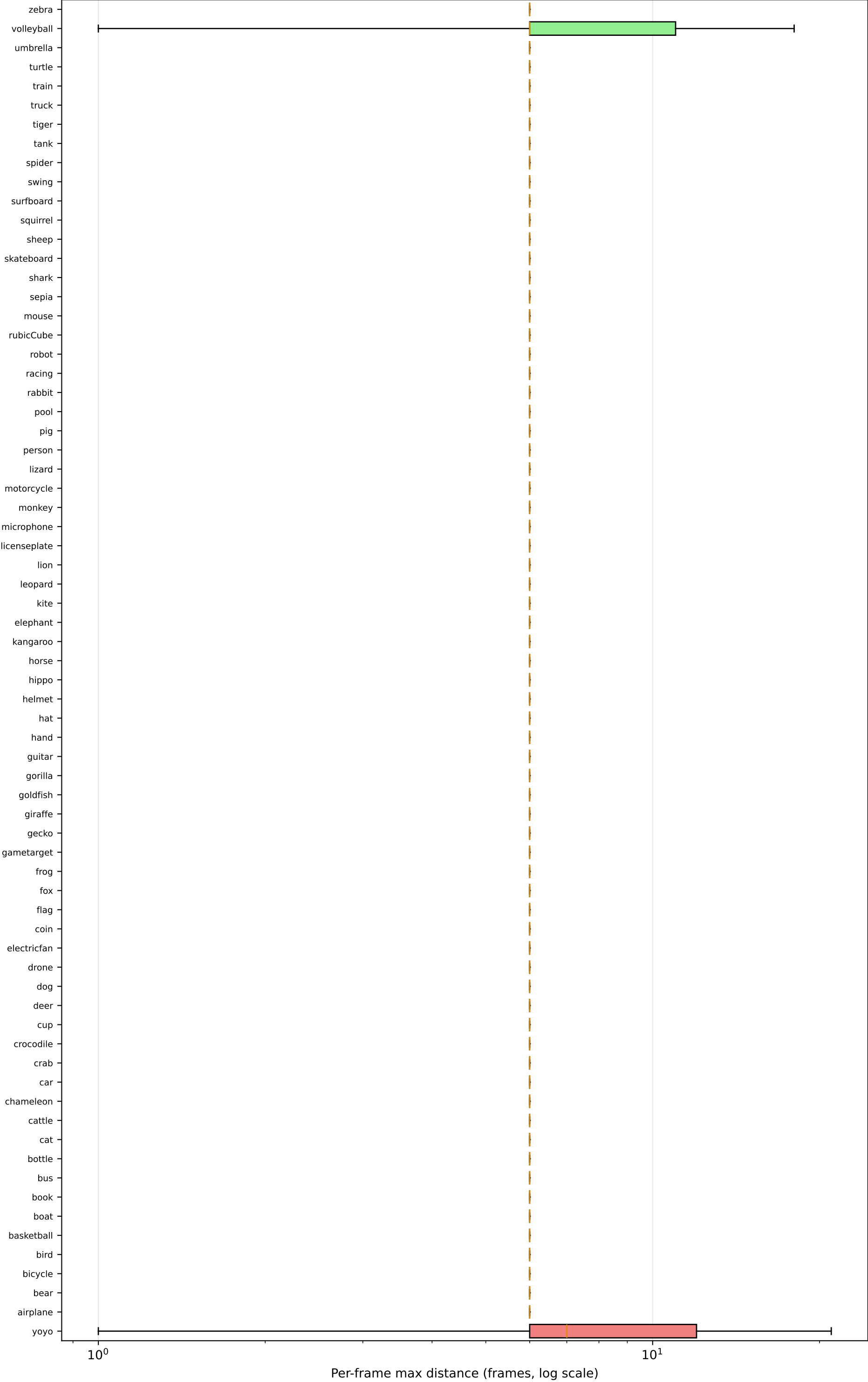
Per-Category Distance Distribution (70 categories, sorted by median)
