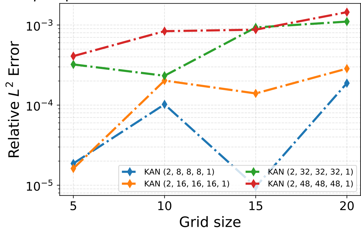
p -Laplacian Obstacle Problem: Error vs. Grid-Size
