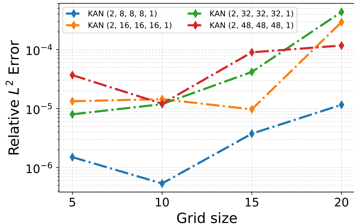
Elastic Obstacle Problem: Error vs. Grid-Size
