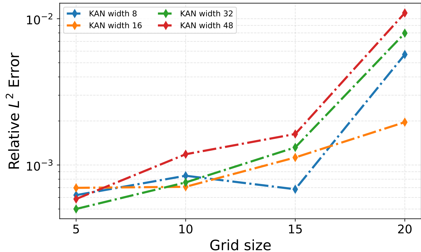
(c) Stefan Problem
