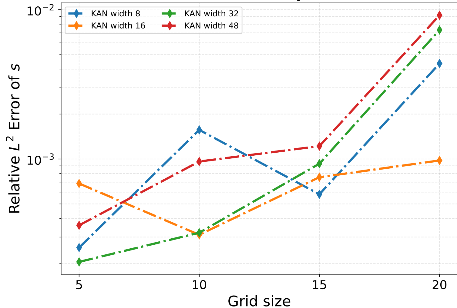
Stefan Problem: Free-Boundary Error vs. Grid-Size
