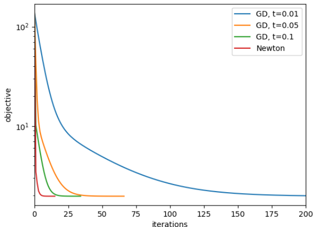
Figure: Comparison between GD and Newton methods. The stopping condition is \|x(k) - x(k-1)\| < 10^{-6} .
