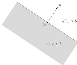
Figure: A hyperplane determines two halfspaces.
