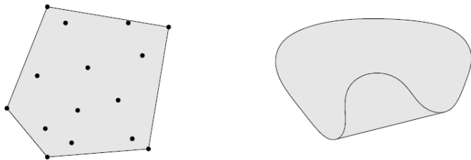
Figure: Some examples of convex hull.
