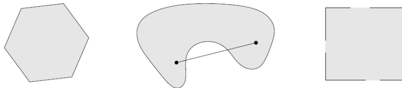
Figure: Left fig. is convex set, middle and right ones are non-convex sets.
