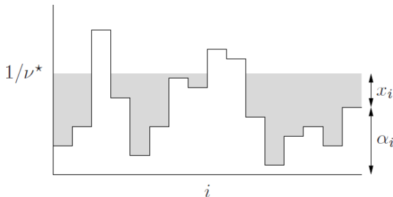
Figure 5.7 Illustration of water-filling algorithm. The height of each patch is given by \alpha_i . The region is flooded to a level 1/\nu^* which uses a total quantity of water equal to one. The height of the water (shown shaded) above each patch is the optimal value of x_i^* .
