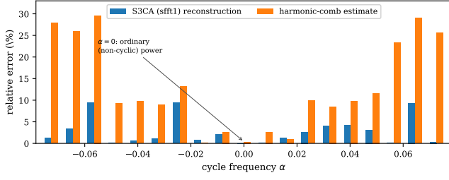
Figure 4: Relative profile-magnitude error, comparing sparse SCD reconstruction and the proposed comb estimator against the dense reference, at each of the 2M_h + 1 = 19 populated cycle frequencies \alpha = m\alpha_0 , m = -9, \dots, 9 (the same locations as Fig. 3). The bar at \alpha = 0 reports error on the ordinary (non-cyclic) power term rather than a harmonic proper. Positive and negative harmonics are shown separately, since the spectral correlation density need not be symmetric in \alpha , and indeed the two sides differ appreciably (e.g. \alpha = 7\alpha_0 versus \alpha = -7\alpha_0 ).
