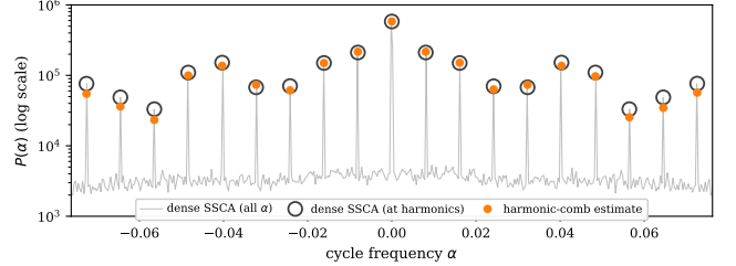
Figure 3: Dense alpha profile compared with the harmonic-comb estimate, on a logarithmic scale. Open circles mark the dense reference value at each harmonic; filled circles mark the estimate at the same location, so that agreement appears as a filled marker centered inside its open ring. The faint background trace is the full dense profile, shown to confirm that no comb location is missed and that the region between harmonics is indeed silent.
