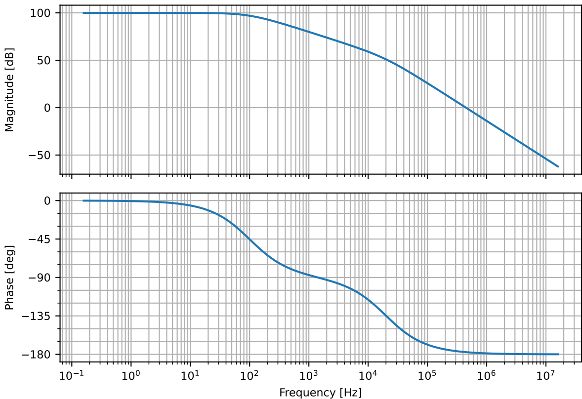
Three Pole Opamp Plot
