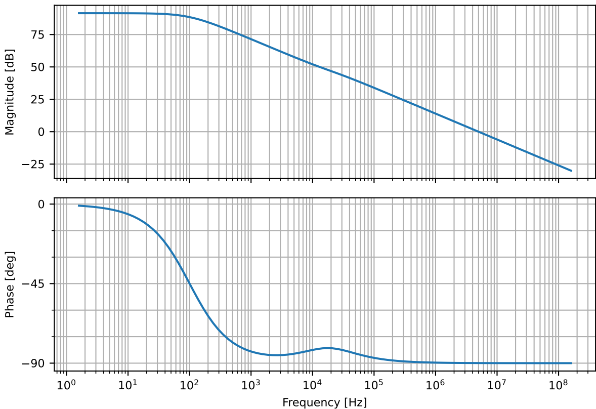
LCR Meter Plot
