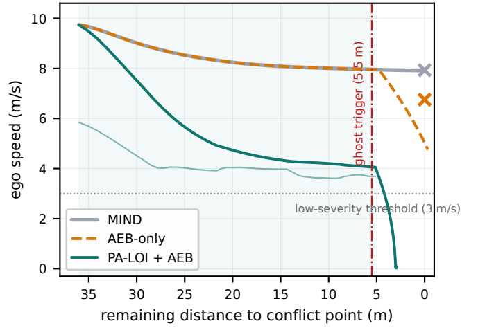
Fig. 5. Mechanism on a representative clean81 scene (index 61, 5.5 m trigger, instant-center): ego speed versus remaining distance to the conflict point, per planning cycle. The thin line under the PA-LOI trace is its active safe-speed bound (7) (shaded span: phantom source active); crosses mark ghost impact speeds; the dash-dotted line is the trigger distance.
