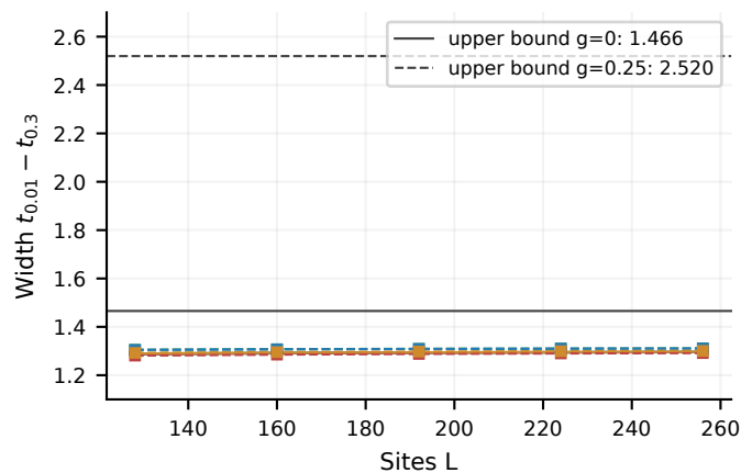
(c) A size-uniform continuous bound
