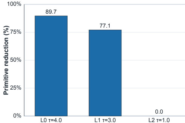
B. Primitive reduction from full detail
