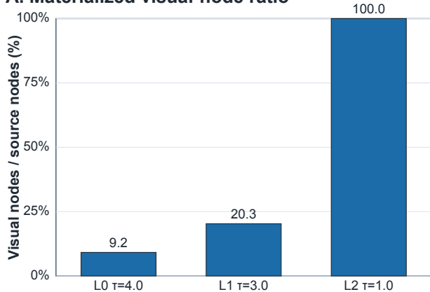
A. Materialized visual-node ratio
