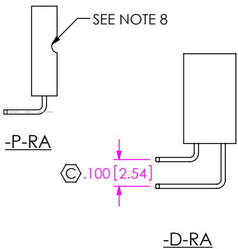
FIG 2 RIGHT ANGLE OPTION ALL OPTIONS DIFFERENT AS SHOWN, OTHERWISE SAME AS -S-RA
