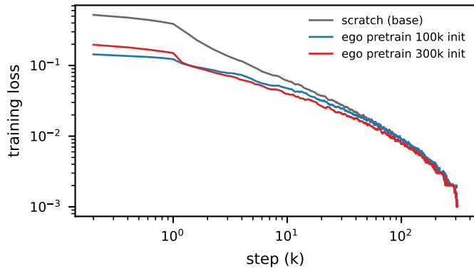
(a) R30 fine-tuning, training loss
