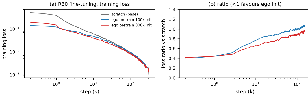
Fig. 6. R30 fine-tuning (30 robot episodes) from the base model and from ego pretraining at 100k and 300k steps. (a) Training loss (log-log, smoothed). (b) Ratio to scratch, shown to 150k; beyond that the 3-decimal losses make the ratio noise. Training loss only, one seed per arm.
