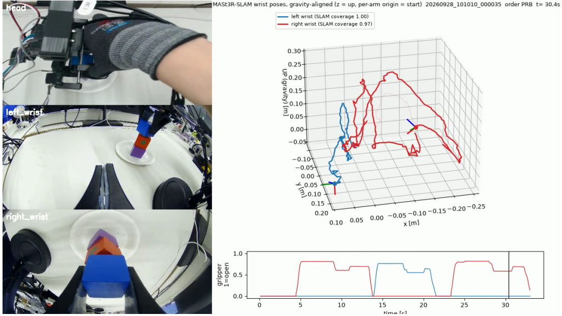
Fig. 4. MAST3R-SLAM wrist trajectories of an HRL80 stacking take (order PRB). Left: head camera and both wrist fisheye cameras. Right: trajectories gravity-aligned (z up), each arm’s origin at its start pose, current tool axes drawn (x red, y green, z blue), metric scale from the IMU; below, both grippers (1 = open). Videos of three takes (PRB, RBP, PBR): docs/media/mast3r_trajectories/hrl80_0000{35,55,60}_wrist.mp4 in the repository.
