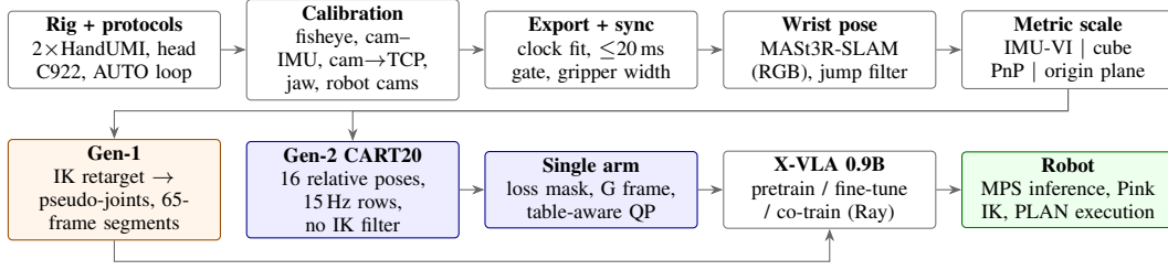
Fig. 1. Pipeline overview. Orange: generation 1 (joint space); blue: generation 2 (Cartesian) and its single-arm variant; green: deployment. Every arrow is followed by a gate with a logged reason.
