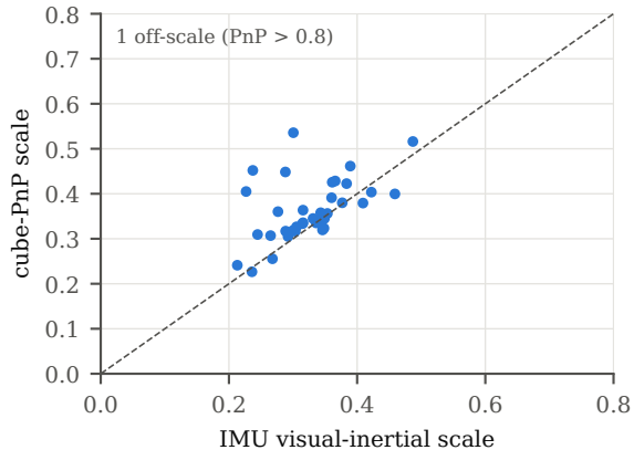
(a) HRL80 takes, 37 PnP-valid: median PnP/IMU 1.06
