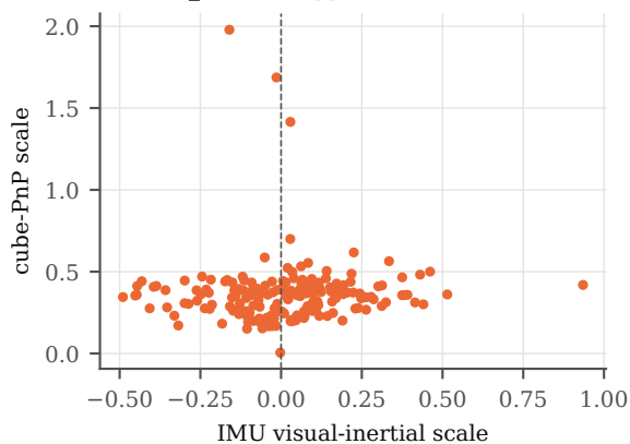
(b) HRA_red slow approaches (181 PnP-valid): IMU scale unobservable
