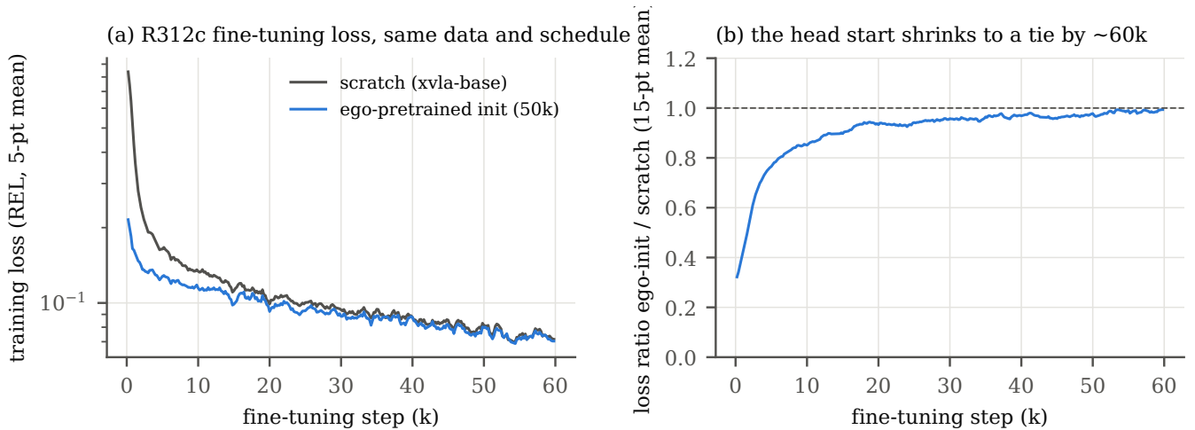
Fig. 4. R312c fine-tuning from the base model versus from the 50k ego checkpoint, same data, schedule and seed. (a) Training loss. (b) Ratio of the two; values below 1 favour the ego initialization. Training loss only.
