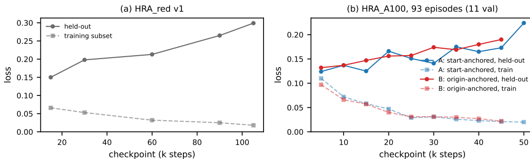
Fig. 3. Held-out (solid) and training-subset (dashed) loss by checkpoint. (a) HRA_red v1, 15 validation takes. (b) HRA_A100, start-anchored (A) and origin-anchored (B) state, 11 validation takes. All runs overfit from the earliest checkpoint.
