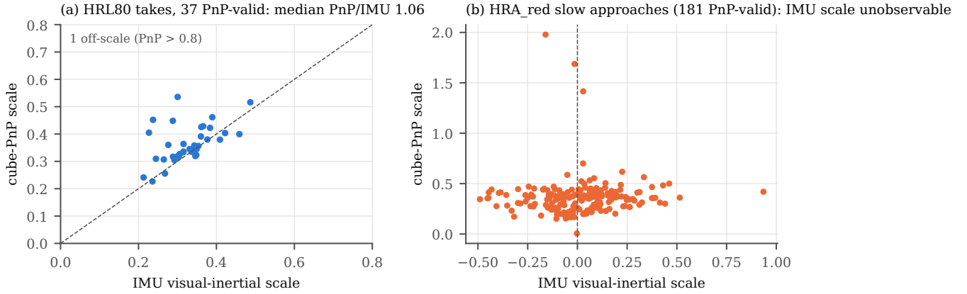
Fig. 1. Per-episode metric scale of the MAST3R-SLAM trajectory from the IMU and from cube PnP. (a) HRL80 stacking takes, where the IMU scale is reliable. (b) HRA_red approach takes: the IMU scale scatters around zero.
