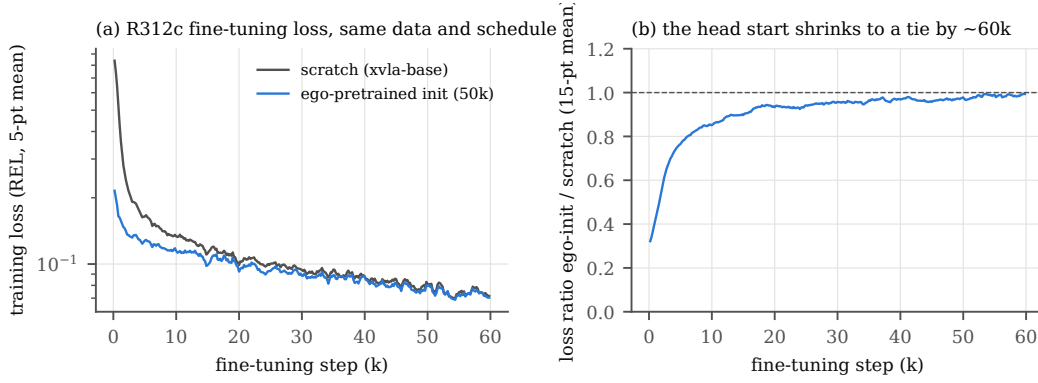
Fig. 3. R312c fine-tuning from the base model versus from the 50k ego checkpoint, same data, schedule and seed. (a) Training loss. (b) Ratio; values below 1 favour the ego initialization.
