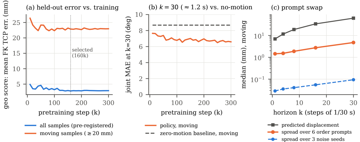
Fig. 2. Generation-1 offline evaluation. (a) Geo score over training, all versus moving samples. (b) Joint MAE at k=30 on moving samples, policy versus zero-motion predictor. (c) Prompt swap: spread across six instructions versus three noise seeds.
