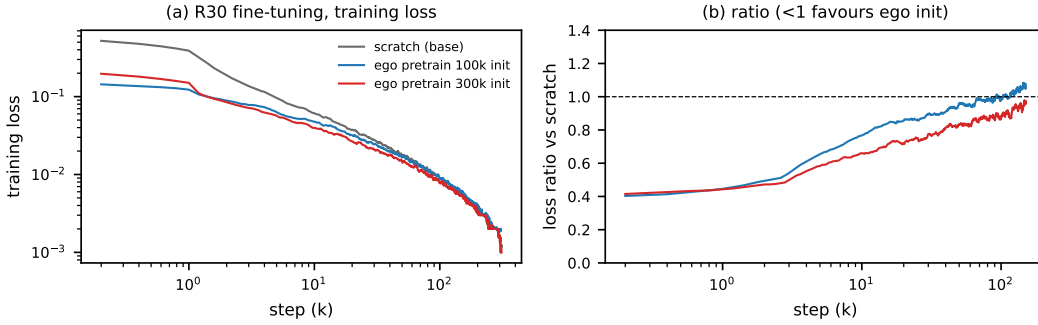
Fig. 4. R30 fine-tuning from the base model and from ego pretraining at 100k and 300k steps. (a) Training loss. (b) Ratio to scratch up to 150k. Training loss only.
