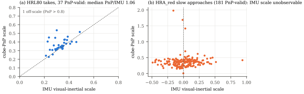
Fig. 1. Per-take metric scale from the IMU and from cube PnP. (a) HRL80 stacking takes, where the IMU is reliable. (b) HRA_red approach takes: the IMU scale scatters around zero.
