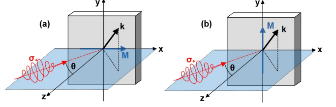
FIG. 1. Symmetry analysis. A circular polarized laser pulse (shown in red, with helicity \sigma_+ impinges onto a magnetic domain (rectangular solid). The light incidence direction and the surface normal ( z -axis) span the scattering plane (blue; xz -plane) with the magnetization direction \mathbf{M} oriented within (a) or perpendicular (b) to the scattering plane, respectively. The off-normal detection of photoelectrons with wavevector \mathbf{k} (black arrow) results in a chiral setup.
