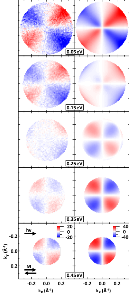
FIG. 2. Momentum-resolved polarization asymmetry A_{\text{pol}} of Fe(001) at selected binding energies for 65° grazing light incidence. Left column: experimental results. The arrow marked h\nu indicates the light incidence direction. The arrows M represent the two magnetization directions considered for A_{\text{pol}} . Right column: respective theoretical results obtained from photoemission calculations. The binding energy is indicated at each panel. The color scale, showing A_{\text{pol}} as defined in Eq. (2a) in percent, is identical for all panels in a column.
