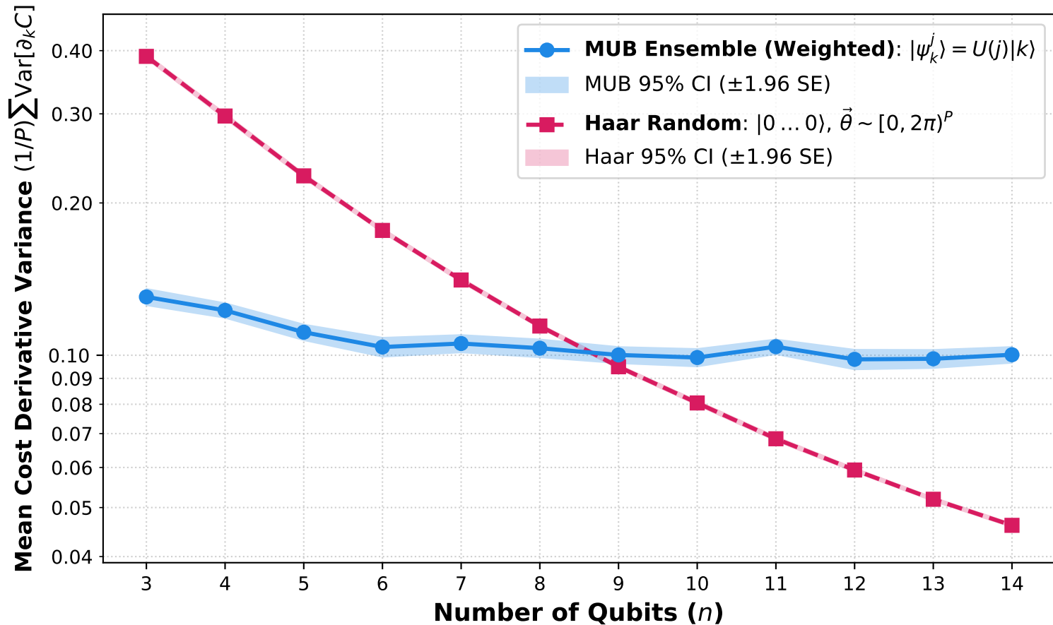
VQE Mean Cost Derivative Variance vs. System Size n All-to-All DM Model ( J_x=1.0 , J_y=0.5 , D=0.8 , h=1.0 , 1/n ) HEA Depth L = 2n , (1/P)\sum \text{Var}[\partial_k C] ( N = 10000 samples)
