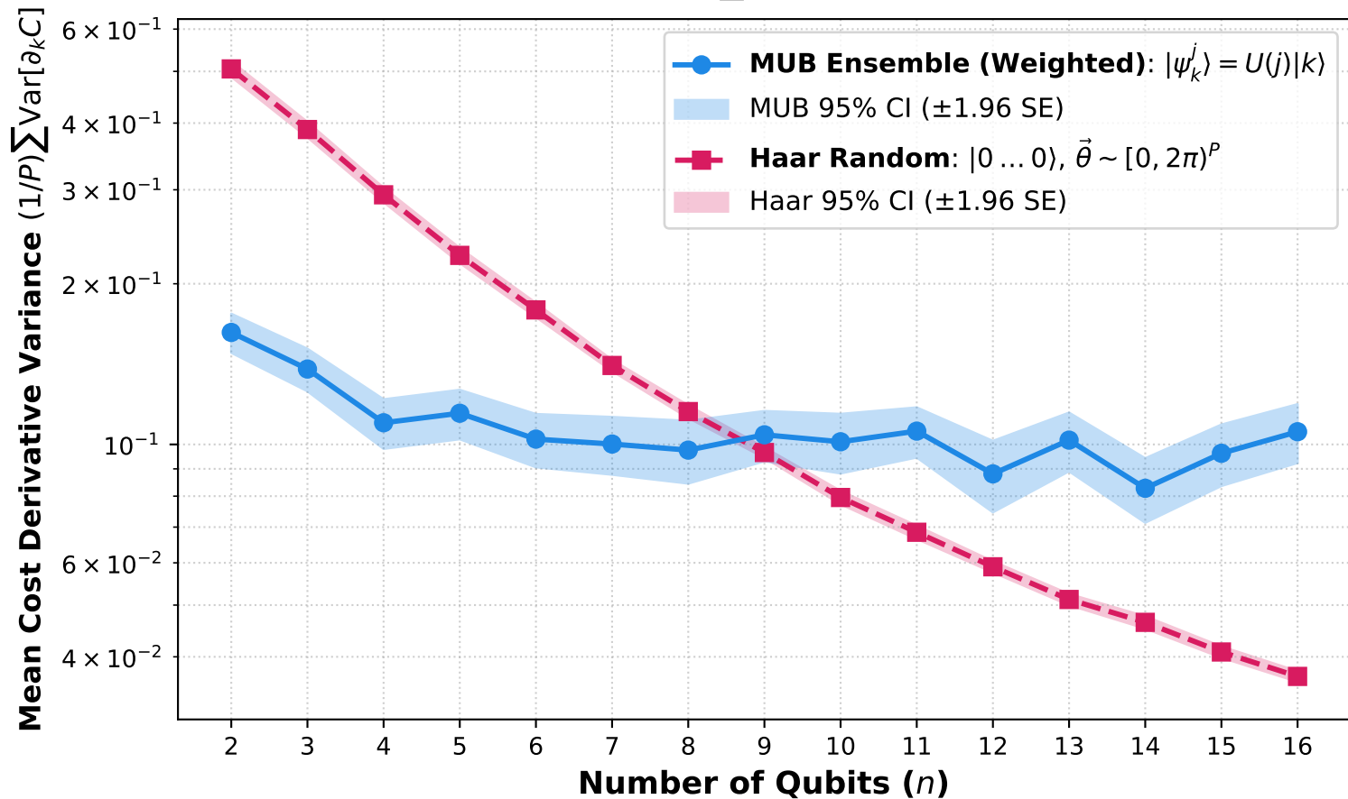
VQE Mean Cost Derivative Variance vs. System Size n All-to-All DM Model ( J_x=1.0 , J_y=0.5 , D=0.8 , h=1.0 , 1/n ) HEA Depth L = 2n , (1/P)\sum \text{Var}[\partial_k C] ( N = 1000 samples)
