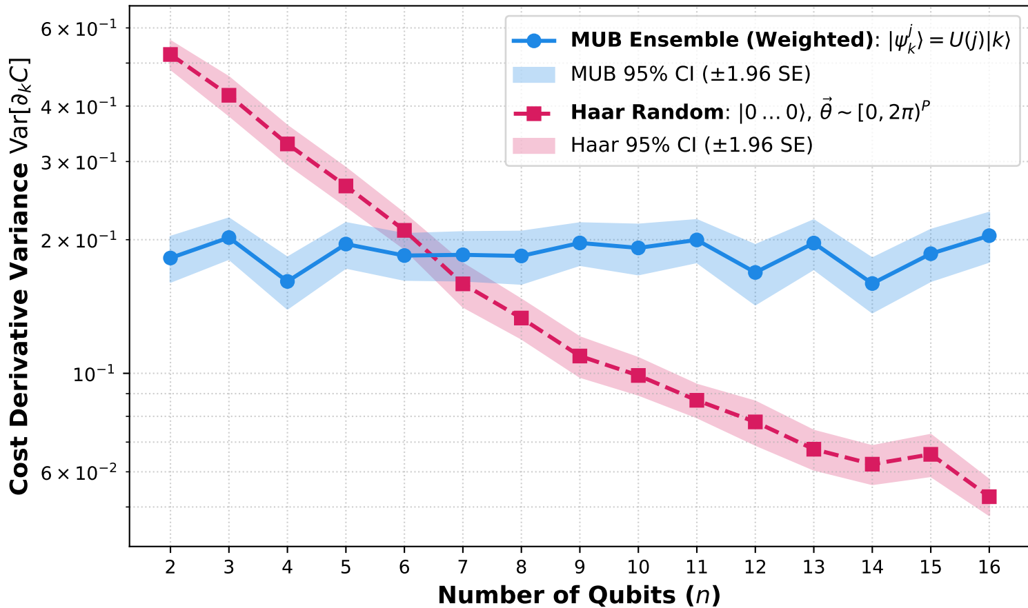
VQE Cost Derivative Variance vs. System Size n All-to-All DM Model ( J_x=1.0 , J_y=0.5 , D=0.8 , h=1.0 , 1/n ) HEA Depth L = 2n , Parameter \partial_{\theta_1} C
