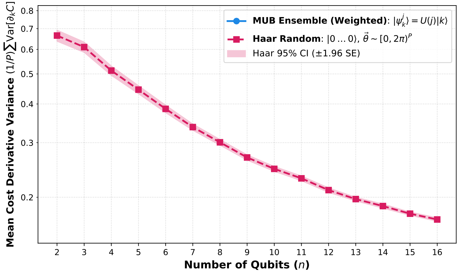
VQE Mean Cost Derivative Variance vs. System Size n 1D Classical Ising Model ( J = 1.0, h = 1.0, ZZ + Z ) HEA Depth L = 2n , (1/P)\sum \text{Var}[\partial_k C] ( N = 1000 samples)
