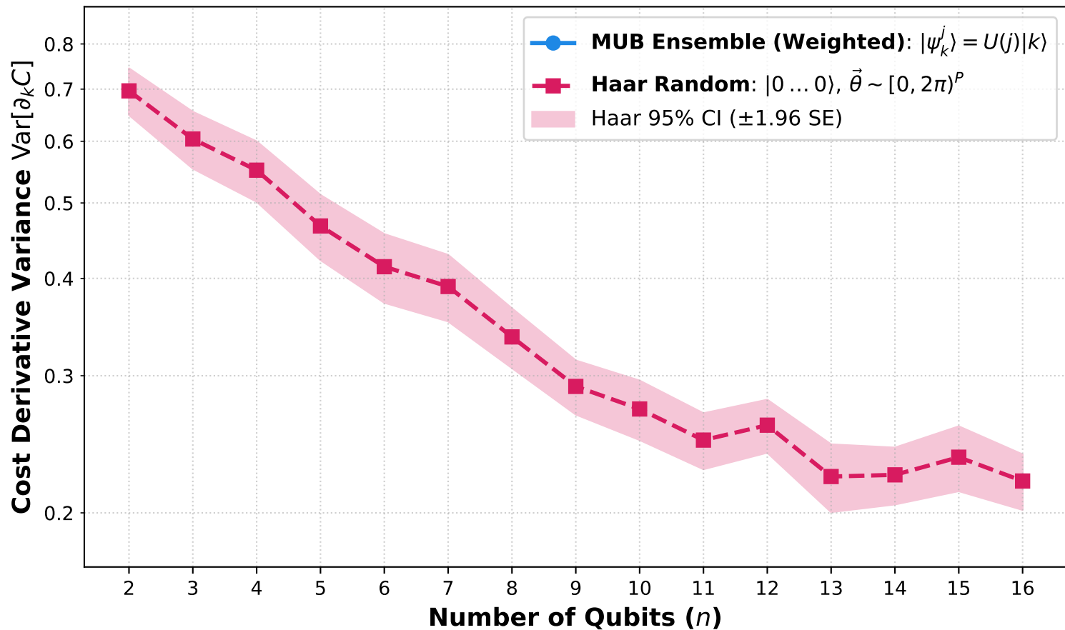
VQE Cost Derivative Variance vs. System Size n 1D Classical Ising Model ( J = 1.0, h = 1.0, ZZ + Z ) HEA Depth L = 2n , Parameter \partial_{\theta_1} C
